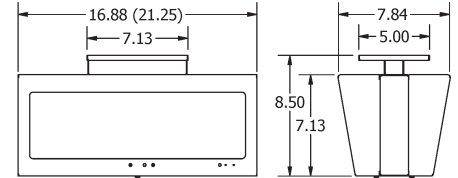
DF-DW400-4 (DF-DW400-6) Ceiling Mount
