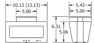
DF-DW225-4 (DF-DW225-6) Ceiling Mount
